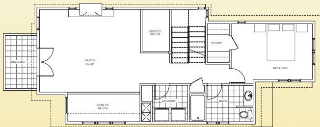
second floor
